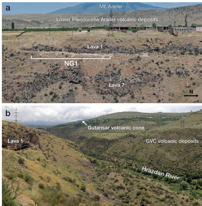
Fig. 2. (a) Photograph of NG1, looking toward the west from the eastern side of the Hrazdan valley, and the associated geomorphological features. (b) Photograph of the Hrazdan valley, looking north-east from NG1, showing the visibility of the Gutansar cone. Photographs by the authors.
