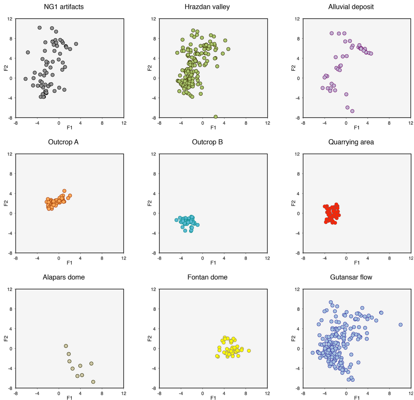
Fig. 10. Scatterplots of the first and second discriminant functions applied to the magnetic data for the different obsidian sampling areas.
