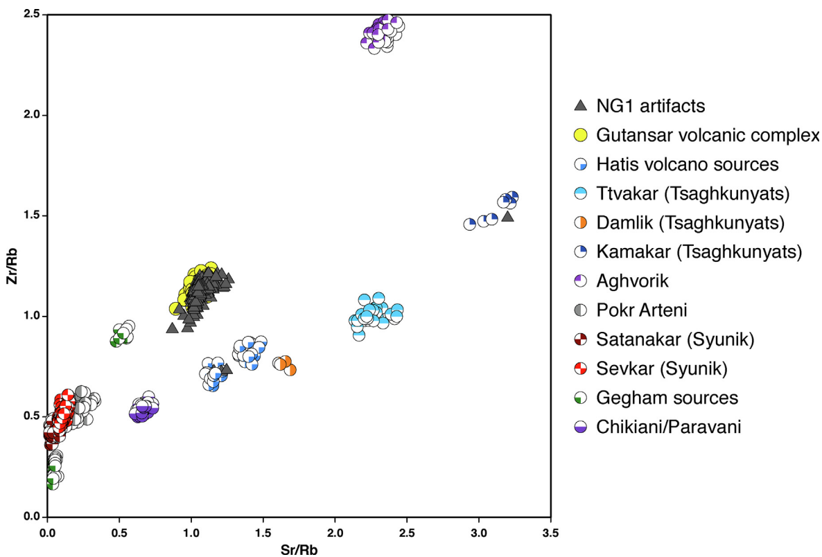
Fig. 9. A scatterplot of Sr/Rb vs. Zr/Rb (i.e., Sr vs. Zr normalized to Rb) for the geological obsidian specimens and the NG1 small debris in this study. This scatterplot is directly comparable to Fig. 7a in Frahm et al. (2016:84).
