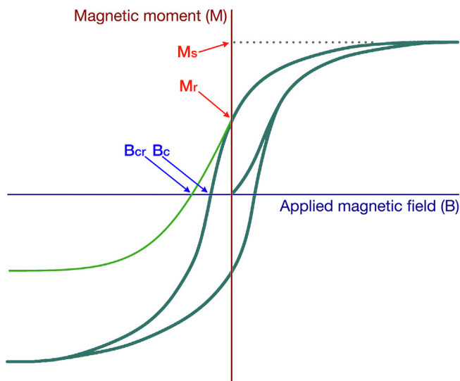
Fig. 7. A generic hysteresis loop after processing (i.e., after the paramagnetic contribution from the glass has been subtracted), illustrating the relationships among the applied magnetic field ( B ); the specimen's magnetic moment ( M ) in response; and the measurement of remanence ( M_r ), saturation magnetization ( M_s ), coercivity ( B_c ), and coercivity of remanence ( B_{cr} ).
