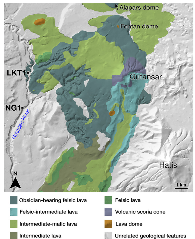
Fig. 3. Redrawn version of the geological map for the Gutansar volcanic complex from Sherriff et al. (2019), largely based on that of Karapetian and Karapetian (1971).
