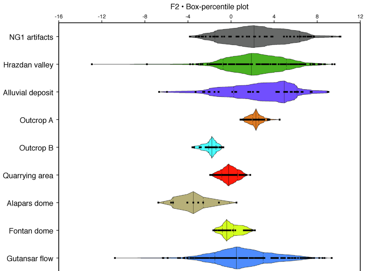
Fig. 12. A box-percentile plot (Esty and Banfield, 2003) of the second discriminant function applied to the magnetic data for the different obsidian sampling areas.
