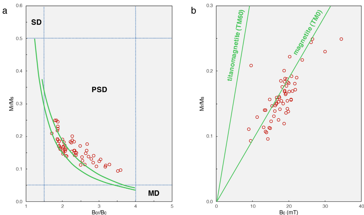
Fig. 8. (a) Day plot ( B_{cr}/B_c vs. M_r/M_s ) of the NG1 obsidian artifacts with magnetic domain boundaries (dotted blue lines) and magnetite mixing curves (solid green lines) from Dunlop (2002). All artifacts fall in the pseudo-single domain (PSD) region of the plot, not the single domain (SD) or multi-domain (MD) regions. Magnetite grains exhibit PSD behavior in the 0.1 to 20 \mu\text{m} size range. (b) NG1 artifact data ( B_c vs. M_r/M_s ) with the compositional lines for magnetite (TM0) and titanomagnetite (TM60) based on calculations by Wang and Van der Voo (2004).
