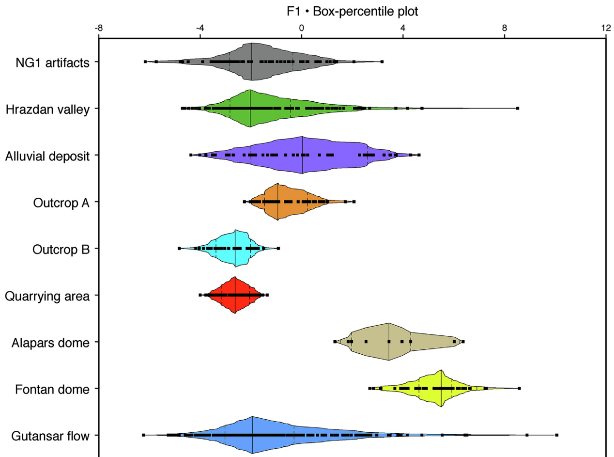
Fig. 11. A box-percentile plot (Esty and Banfield, 2003) of the first discriminant function applied to the magnetic data for the different obsidian sampling areas.
