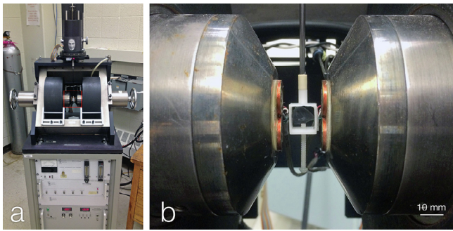
Fig. 6. (a) The vibrating sample magnetometer (VSM) used in this study. (b) A close-up photograph of an obsidian artifact held by a plastic sample holder between the two electromagnetic pole pieces and field sensors. Photographs by the authors.
